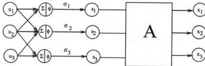
Figure 1: Topographic ICA model [HH01]. The variance generated variables u_i are randomly generated, and mixed linearly inside their topographic neighborhoods. This forms the input to nonlinearity \phi , thus giving the local variance \sigma_i . Components s_i are generated with variances \sigma_i . The observed variables are x_i obtained as with standard ICA from the linear mixture of the components s_i .
