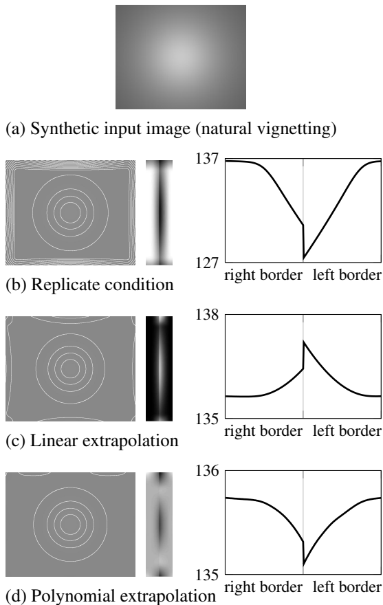
Figure 1: Illumination correction without texture. The intensity levels of the corrected images (left) are emphasised with contours. Additionally, an image transition (middle column, 128 pixels from each side, intensity stretched to full range) and the intensity across the middle row (right) are shown. Note the different scales on the y-axis and that the boundary artifacts are reduced.
